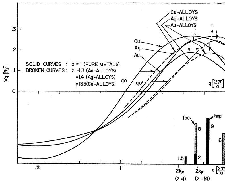
FIG. 3. Fourier expansion of the pseudo-potential of Cu, Ag, and Au (data taken from a recent compilation of Cohen and Heine 10 ), and extrapolated Fourier expansions of the pseudopotentials of Cu, Ag and Au based alloys at the beginning of the hcp phase ( z=1.35 for Cu-alloys, 1.4 for Ag-alloys and 1.3 for Au-alloys). Also shown are the locations of the first few reciprocal-lattice vectors of the fcc and hcp structures with their structural weight, as well as twice the Fermi wave vector for free electrons for z=1 and z=1.4 .
